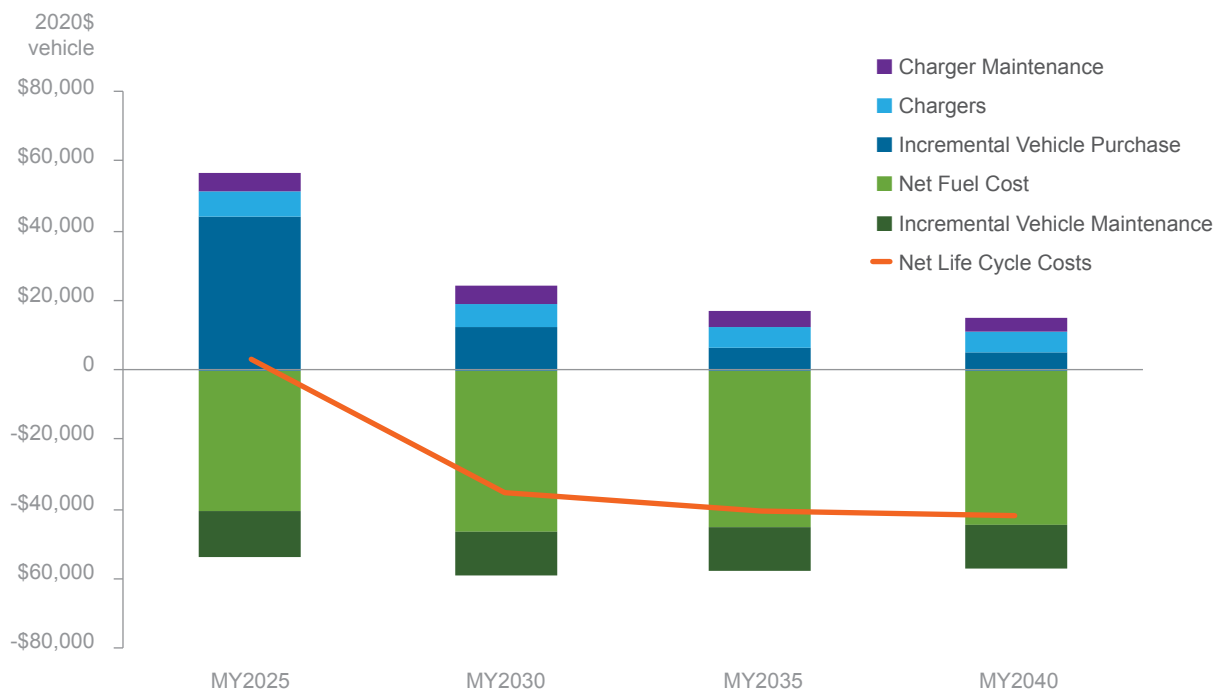
Figure 6 Projected Lifetime Incremental Costs for New Mexico ZEVs Compared with Combustion Vehicles
